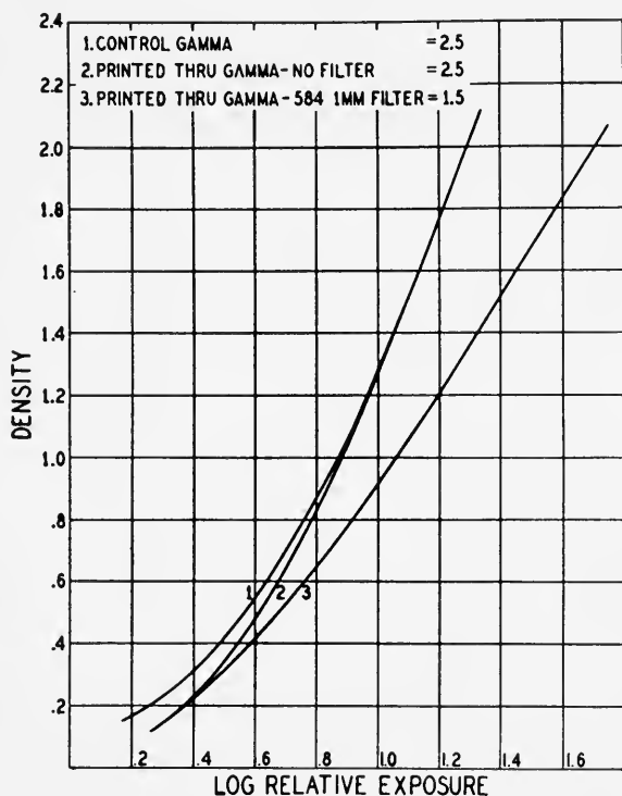
FIG. 6. Effect of ultraviolet filter on sound positive gamma.
